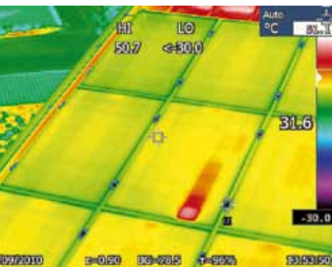
A typical defective spot on a PV module. A thermal imaging camera makes „hot spots“ visible
